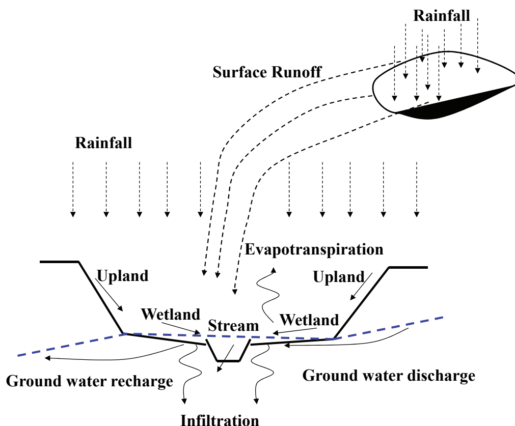
Figure 4.2: Surface/Ground Water Interactions in a Constructed Wetland
